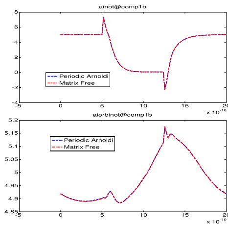
Fig. 12. PSS waveform accuracy comparison at two nodes of a CMOS switch cap. The red line is the nonstructured MF-GMRES, and the blue line is the structured PAS-GMRES.
