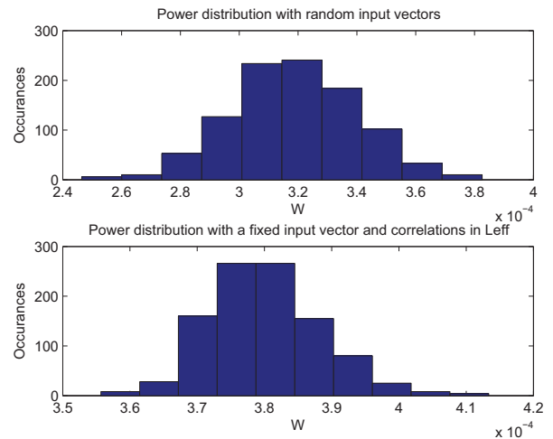
Figure 1: The comparison of circuit total power distribution of circuit c432 in ISCAS'85 benchmark sets (top) under random input vectors (with 0.5 input signal and transition probabilities) and (bottom) under a fixed input vector with effective channel length spatial correlations.
