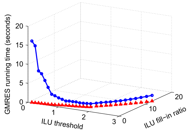
Fig. 14. The impact of ILU threshold on fill-in ratio and GMRES solving time. The blue curve in 3D space is GMRES solving time with respect to threshold and fill-in ratio, and the red curve on the bottom plane reflects the changes of fill-in ratio caused by different threshold values. All the measurements are from ibmpg4t . (For interpretation of the references to color in this figure caption, the reader is referred to the web version of this paper.)
