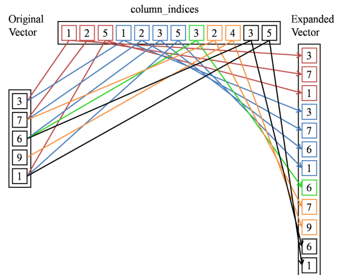
Fig. 8. The vector expansion concept in the P&S method.
