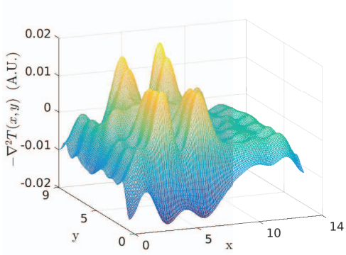
Fig. 3. A negative-Laplacian map example of experiment thermal measurements in 3D view.
