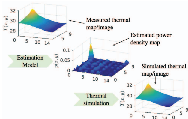
Fig. 8. Setting proper boundary conditions for thermal simulation model using measurements of CPU's idle status
