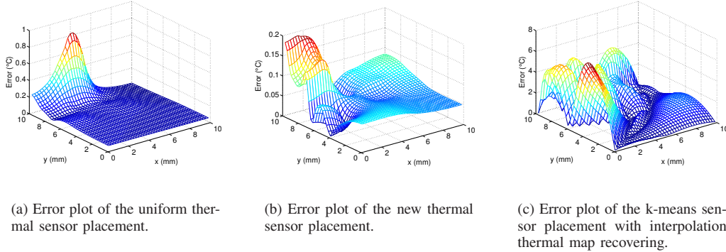
Fig. 4. Error snapshot plot with the bzip2 benchmark at 15s. For both cases, 6 thermal sensors are placed on chip.
