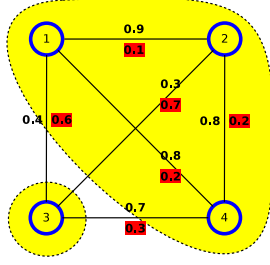
Fig. 2. A correlation clustering example for a complete undirected weighted graph with four vertices. On each edge e_{ij} , w_{ij}^- is shown as red shaded while w_{ij}^+ is in normal. The outputted clusters are surrounded by dashed lines filled with yellow color.
