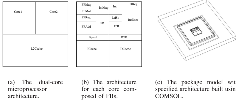
Fig. 3. The dual-core microprocessor architecture, with two cores and one shared L2 cache, and the package model built using COMSOL.
