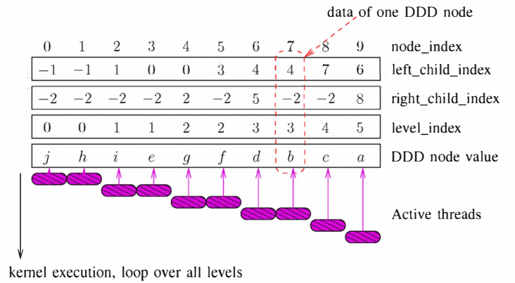
Fig. 3: Leveled continuous storage of a DDD, and levelwise GPU evaluation of the DDD in Fig. 1.
