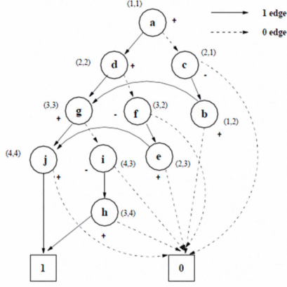
Fig. 1: DDD representation for matrix M .
