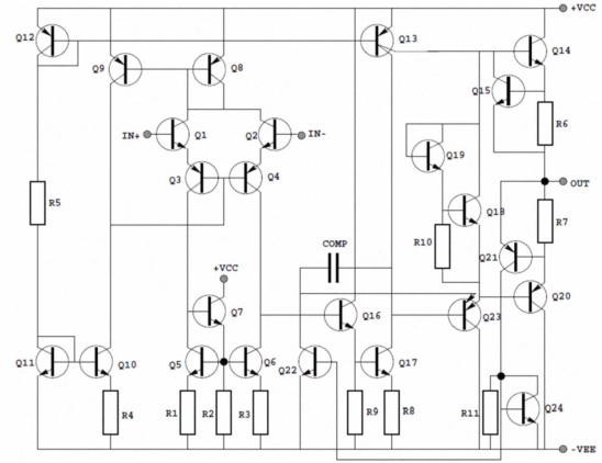
Fig. 5: The circuit schematic of \mu A741
