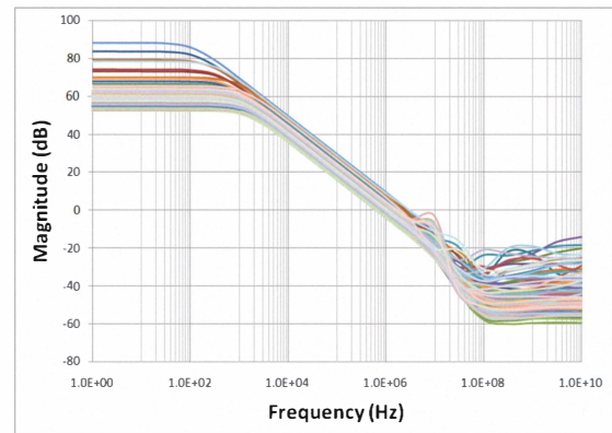
Fig. 7: The cluster of frequency responses of the tested \mu A741 circuit
