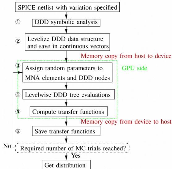
Fig. 2: The flow of GPU-based parallel Monte Carlo analysis.
