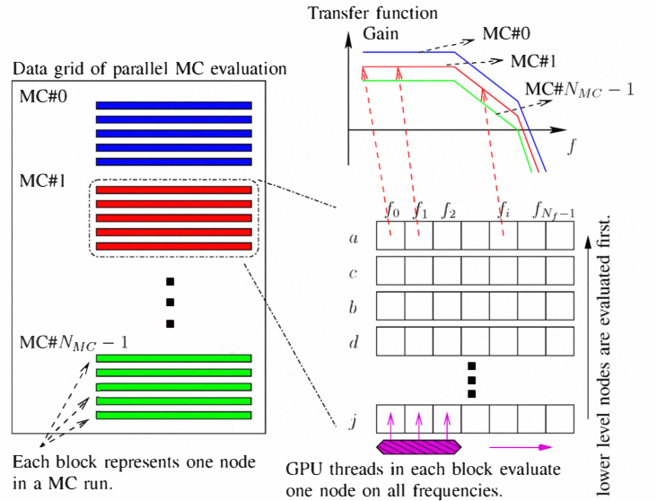
Fig. 4: GPU parallel evaluation of the DDD in Fig. 1.
