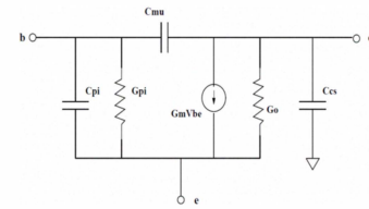
Fig. 6: The small signal model for bipolar transistor
