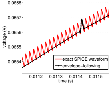
(b) Detail of one EF simulation period
