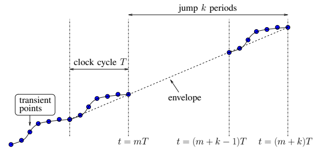
(a) Illustration of one envelope skip.
