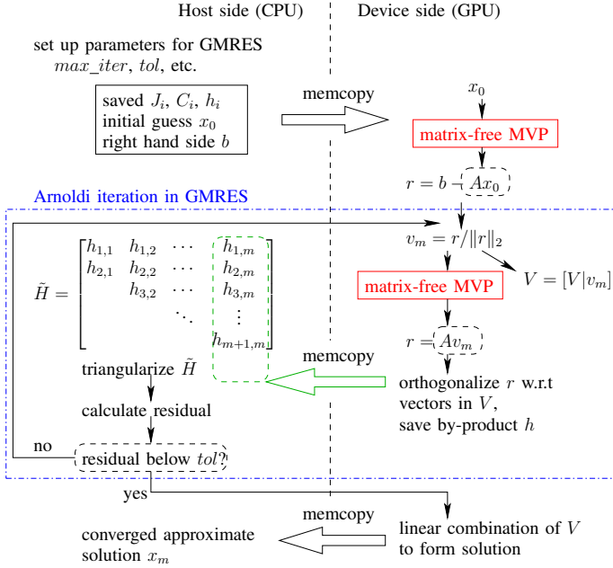
Fig. 3. GPU parallel solver for envelope-following update.
