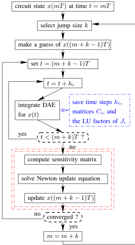
Fig. 2. The flow of envelope-following method.
