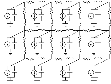
Fig. 5. Illustration of power/ground network model.
