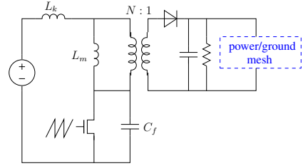
Fig. 4. Diagram of a zero-voltage quasi-resonant flyback converter.
