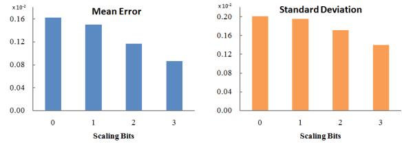
Figure 8: The mean error and standard deviation of 8-bit Scaled-CBSC multiplication approach.
