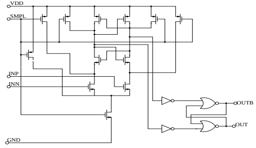
Figure 9: The MOS circuit implementation for the comparator.
