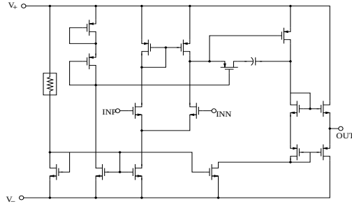
Figure 7: The MOS circuit implementation for the OPAMP.
