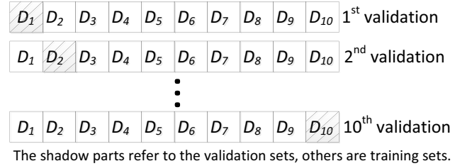
Fig. 4: The algorithm processing chart of 10-fold cross-validation.
